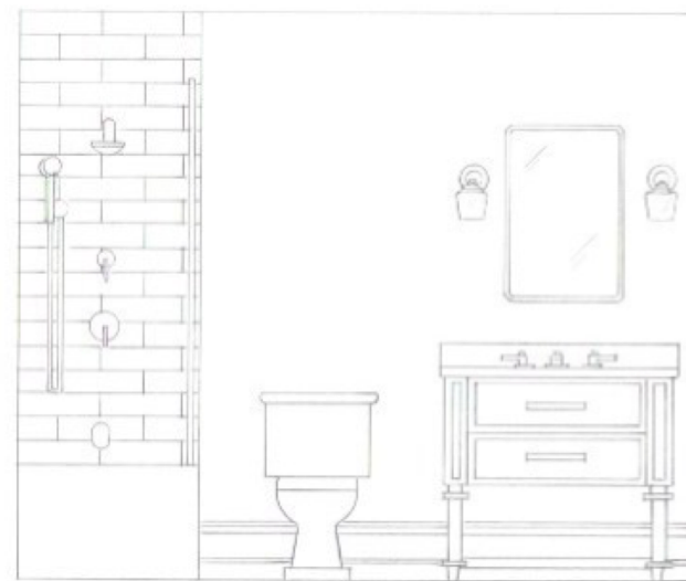
DEAN BATH - VANITY ELEVATION SCALE - 1/2" = 1'-0"
