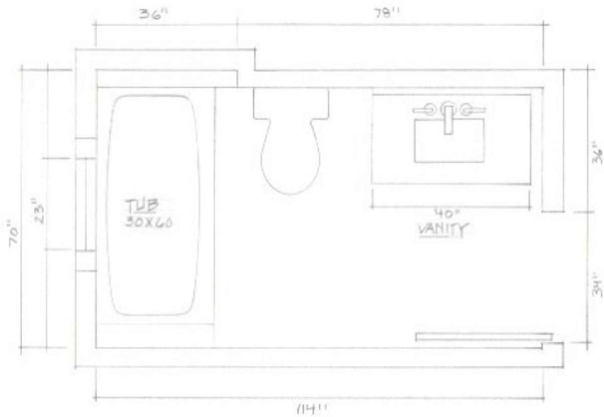
DEAN BATH SCALE - 1/2" = 1'-0"
